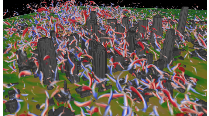
Visualizing turbulence structures within the urban canopy
