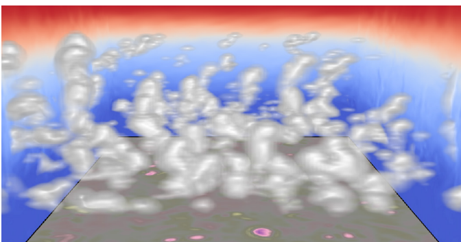
Shallow cumulus clouds from the BOMEX model intercomparison
