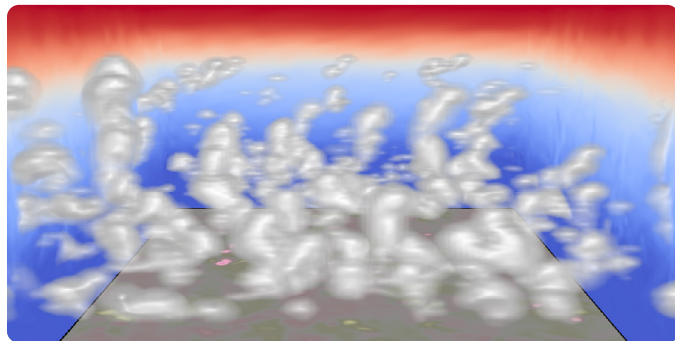
Shallow cumulus clouds from BOMEX model intercomparison
