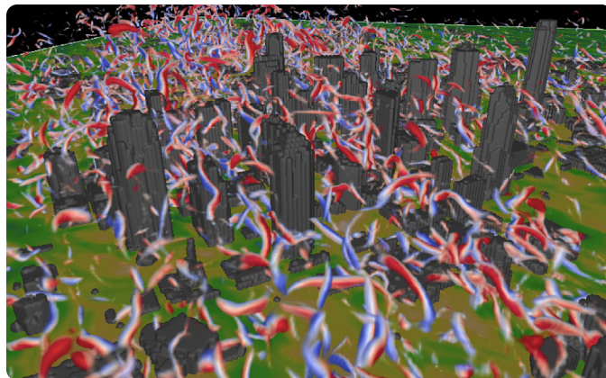
Visualizing turbulence structures within the urban canopy
